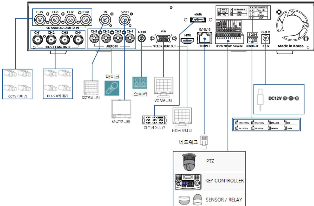
[Figure 2-1. SVR-1004HDL Basic Connection and Device Connection]
